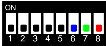
Fig 3. RX35X INSTALLATION INSTRUCTIONS PCB Connections
