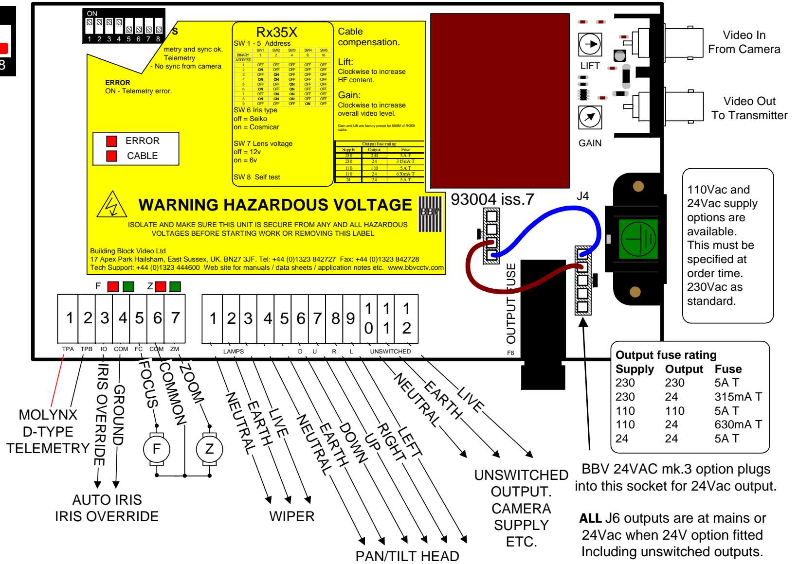
Fig 3. RX35X INSTALLATION INSTRUCTIONS PCB Connections
